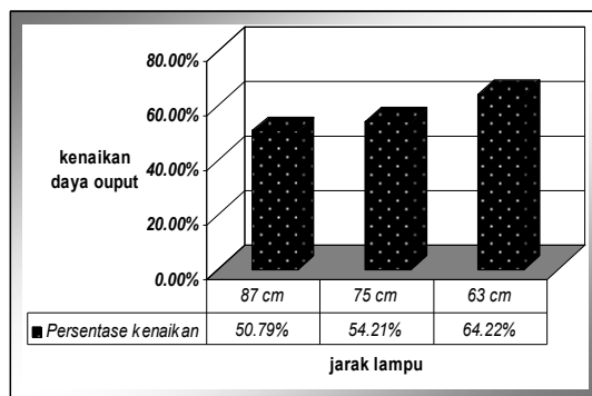
Gambar 6. diagram persentase kenaikan daya output modul surya
