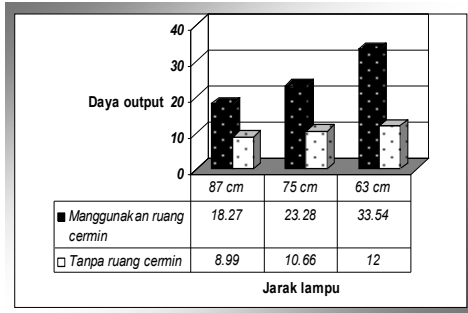
Gambar 5. diagram perbandingan daya output modul surya
