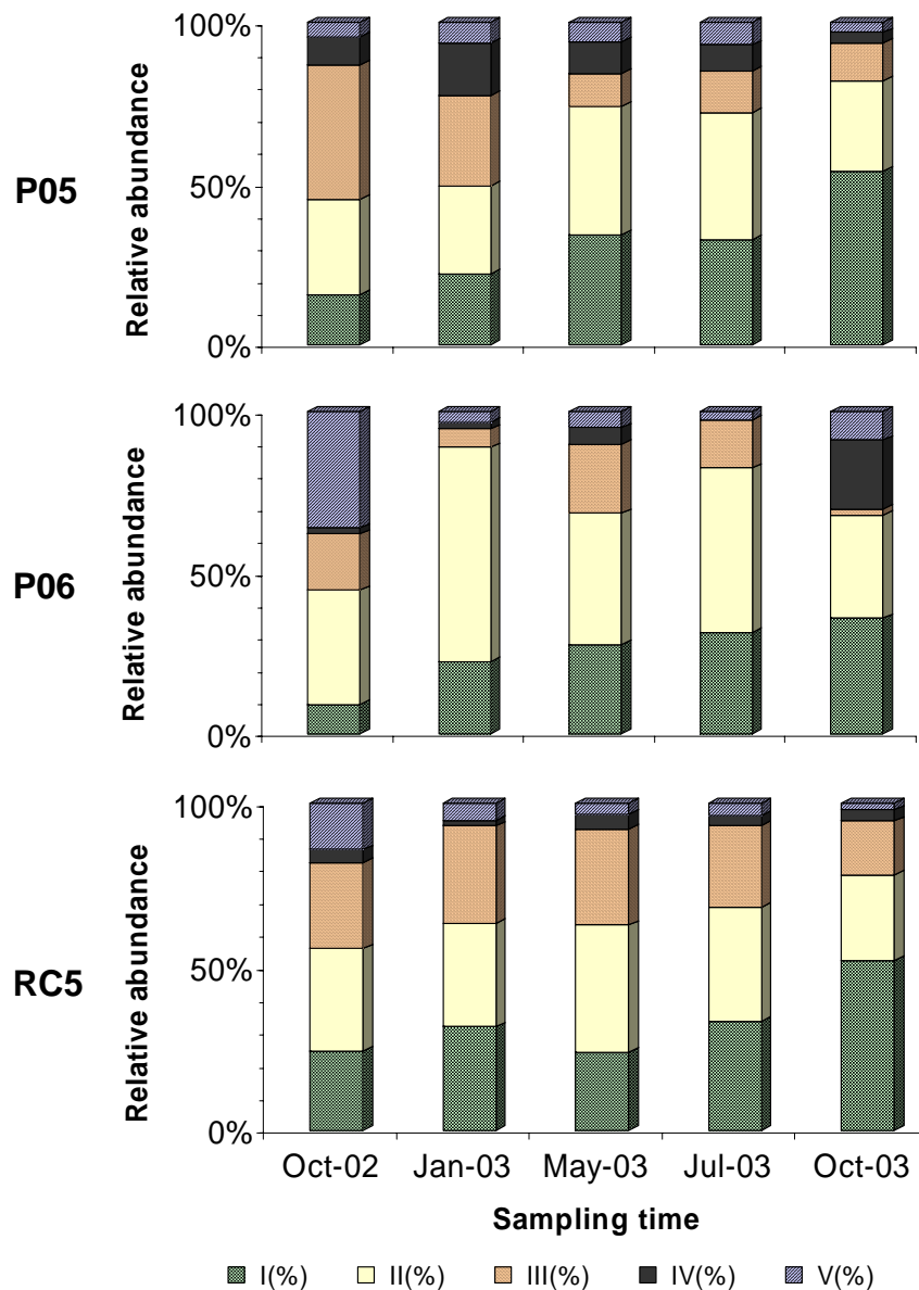
Fig. 2. Relative abundance of the ecological groups of three selected sites, based on the AMBI, over the study period.
