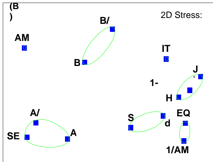
Fig. 1. Dendrograms (A) and MDS plots in 2 dimensions (B) of biotic indices derived from Spearman rank correlation coefficient matrix of square root transformed data. Green circles derived from cluster analysis, indicate an arbitrary correlation level of 0.7.
