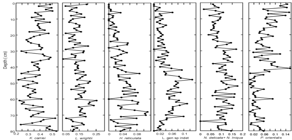
Fig. 4. Temporal change of dominant species
