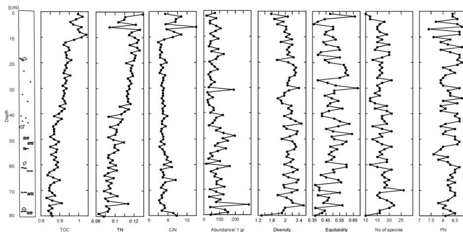
Fig. 2. Temporal changes of composition of ostracode assemblages (abundance, number of species, diversity, equitability) and total organic carbon (TOC) content (wt%), total Nitrogen (TN) content (wt%) and the ratio of TOC/TN contents. Abundance means the number of specimens per 1 gr dry sediment.
