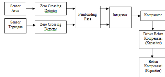
Gambar 12. Blok diagram
