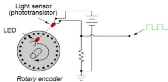
Gambar 2. Sensor optocoupler [7]
