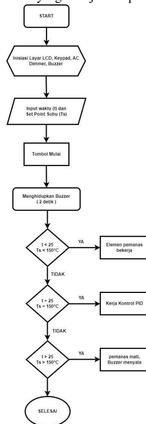
Gambar 4. Flowchart Sistem
