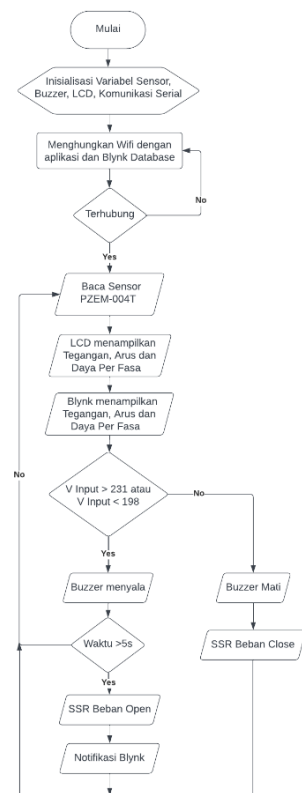
Gambar 4. Flowchart Sistem
