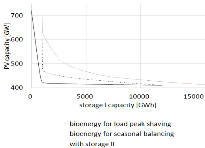
Fig. 8 PV capacity as a function of storage I capacity for systems I, II, and III (system III without charging power limit for storage II)
