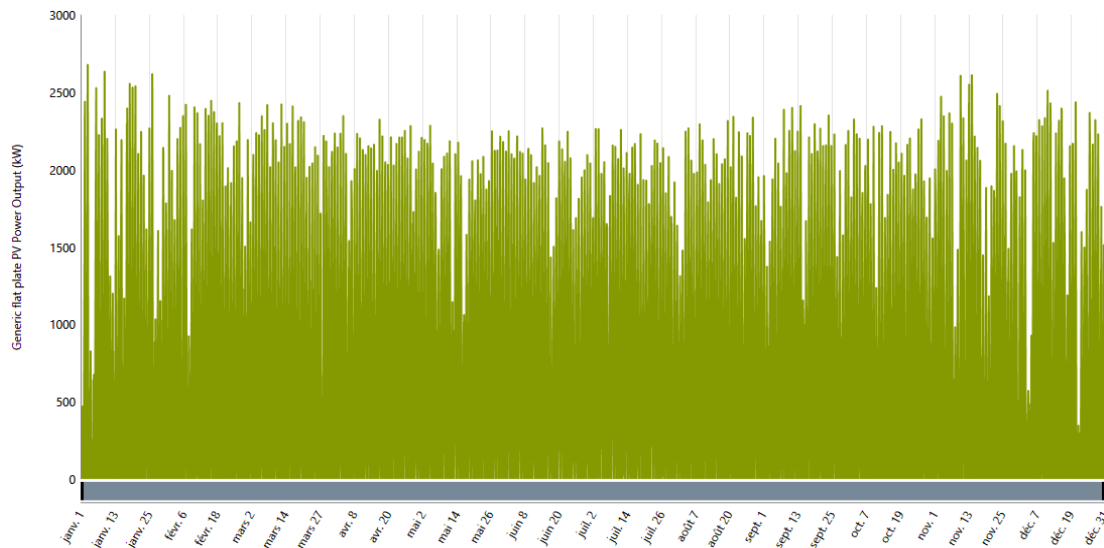
Fig 5. Solar photovoltaic yearly production
