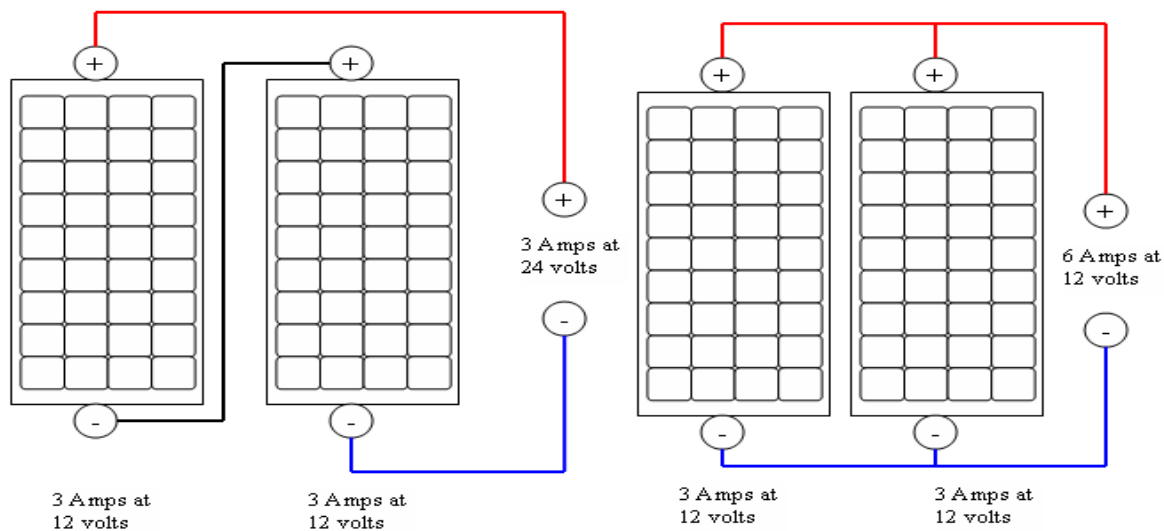
Fig. 3 The connection of PV System in series (left side) and in parallel (right side)
