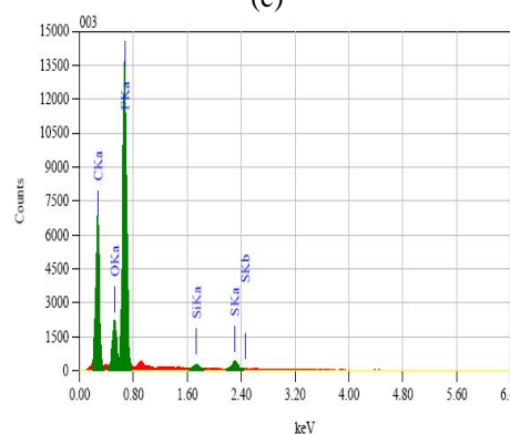
Fig. 3 The EDS pattern of the composite membrane: (a) A1 (pure afion), (b) B1 (R = 0.05 w/w), (c) C1 (R = 0.1 w/w) and (d) F1 (R = 0.05 w/w).
