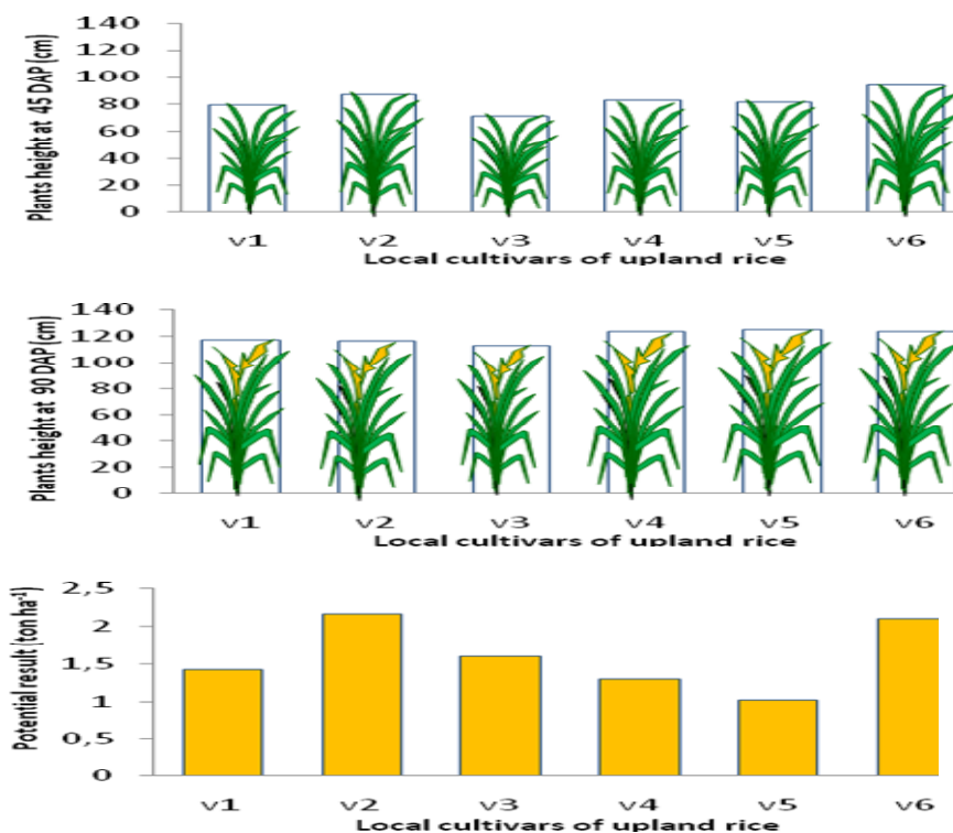
Figure 1. Graph from result of research data summary; a) plants hight when measurement at 45 DAP, b) plants hight when measurement at 90 DAP, and c) result potency six local cultivars up land paddy (ton ha -1 )
