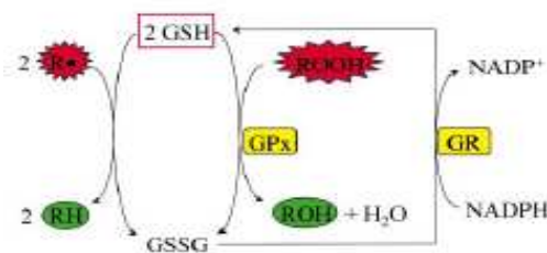
Figure 2. The process of free radical scavenging by glutathione
