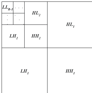
Fig. 1: DWT subband structure
