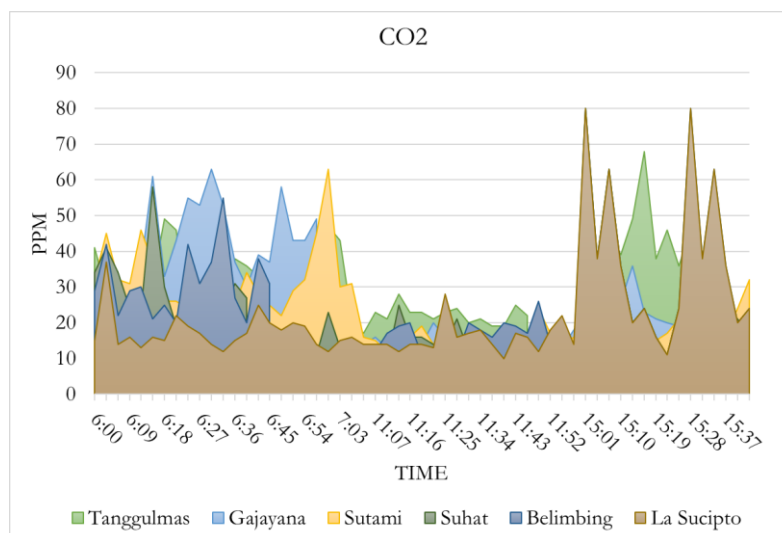
Figure 6. CO 2 Timeline Graph
