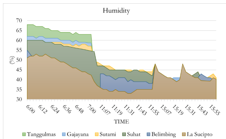
Figure 4. Humidity Timeline Graph
