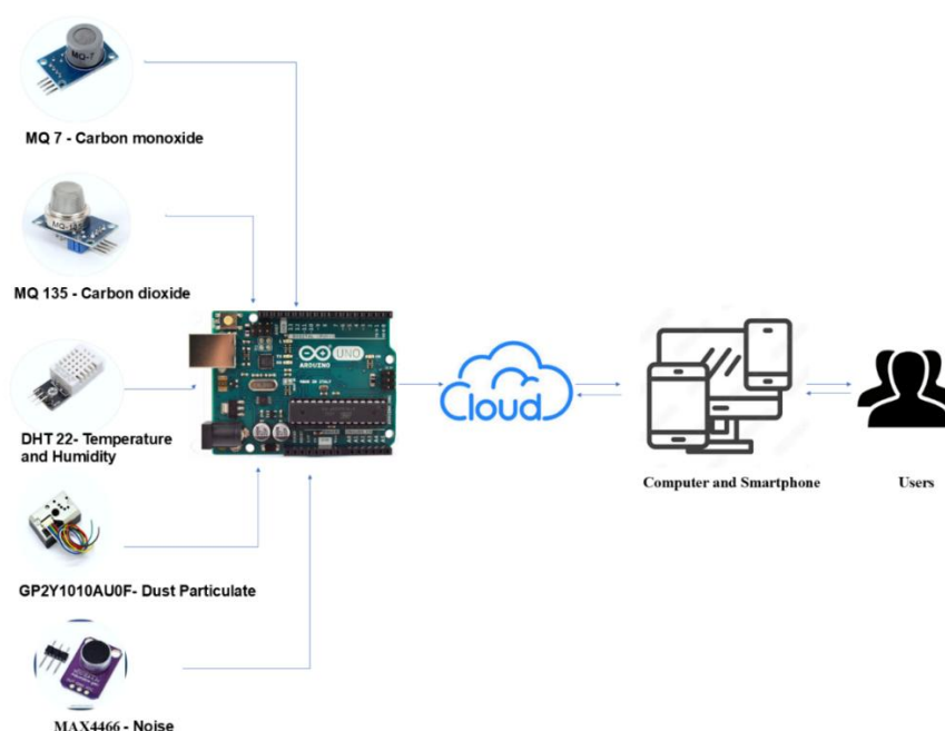
Figure 2. IoT Air Quality Sensing Node Architecture
