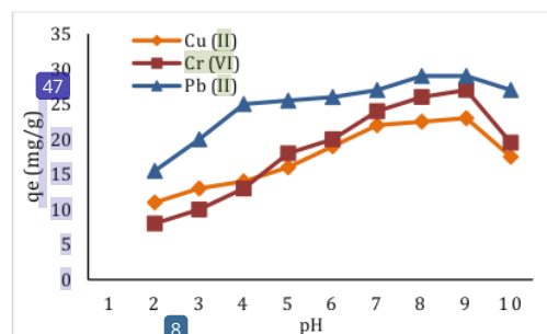
Figure 5. Impact of the solution pH on the sorption of Pb, Cr, and Cu metals (Özsin et al., 2019)
