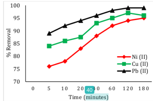
Figure 4. Impact of contact time on the metal ion sorption by papaya peel carbon (Mittal et al., 2021).
