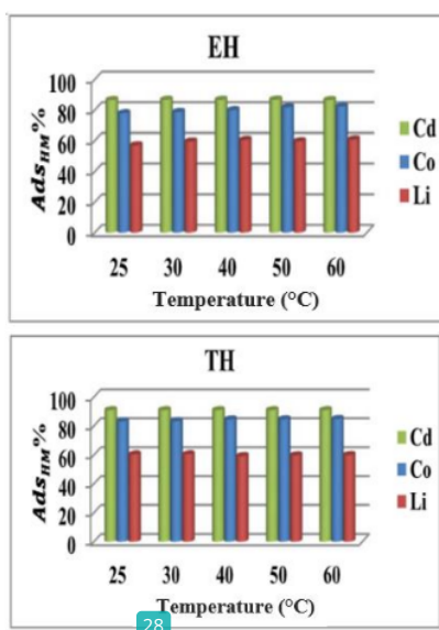
28 Figure 6. The impact of temperature on the removal of metal ions by Equisetum (EH) and Teucrium (TH) adsorbents (Al-Senani & Al-Fawzan, 2018)
