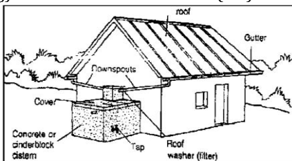
Figure 2. Illustration of the Rainwater Harvesting (PAH) Concept
