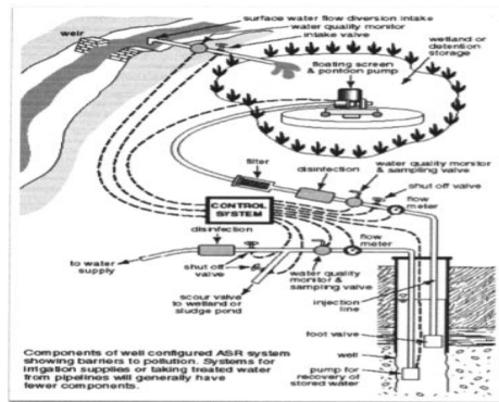
Figure 3. Illustration of the Infiltration Well Concept.
