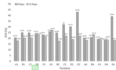
Figure 11. Efficiency of Conversion of Digested Food
