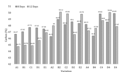
Figure 4. Carbon Content of Residue
