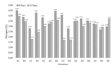
Figure 5. Nitrogen Content of Residue
