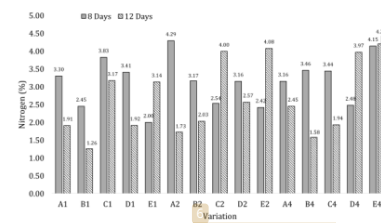
Figure 3. Nitrogen Content of BSF Larvae
