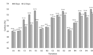
Figure 2. Carbon Content of BSF Larvae
