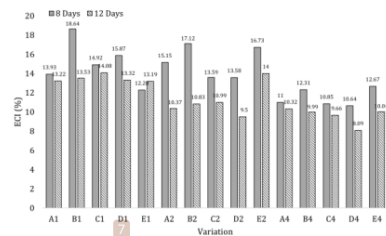
Figure 12. Efficiency of Conversion of Ingested Food Efficiency of Conversion of Ingested Food (ECI) measures the proportion of ingested feed that is utilized for energy production and biomass formation. It is influenced by feed digestibility and the larvae's metabolic efficiency (Permana & Putra, 2018; Waldbauer, 1968). ECI values can be seen on Figure 12. The highest value was observed in substrate B1,
