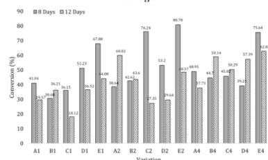
Figure 9. Conversion of Substrate Nitrogen to Residue Nitrogen
