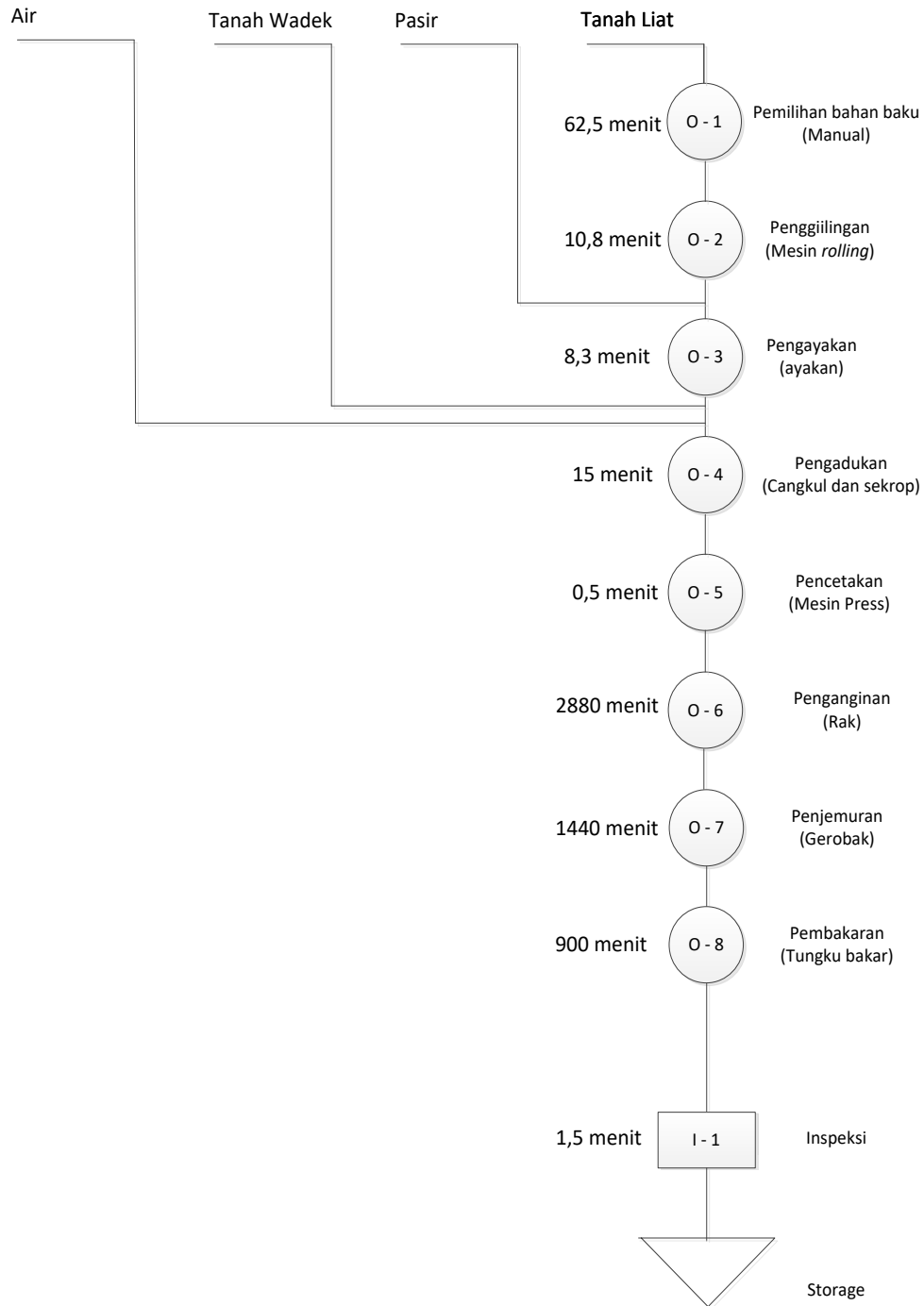
Gambar 1. OPC ( Operation Process Chart )
