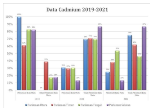
Figure 1. Cadmium Data 2019-2021
