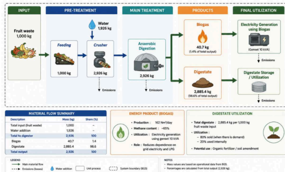
Gambar 1. Material Flow Analysis Proyek BGS
