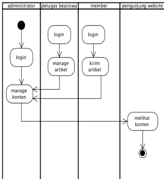
Gambar 3.2 Activity Diagram Manajemen Konten Website
