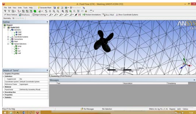
Gambar 6. Hasil mesh
