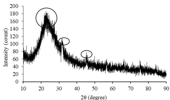
Figure 3. X-ray diffractions analysis (XRD) of purified \text{SiO}_2 of petung bamboo leaf
