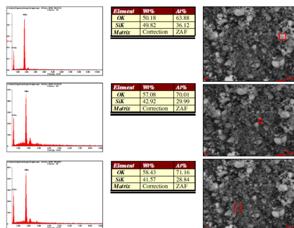
Figure 4. SEM-EDX analysis of purified \text{SiO}_2 of petung bamboo leaf
