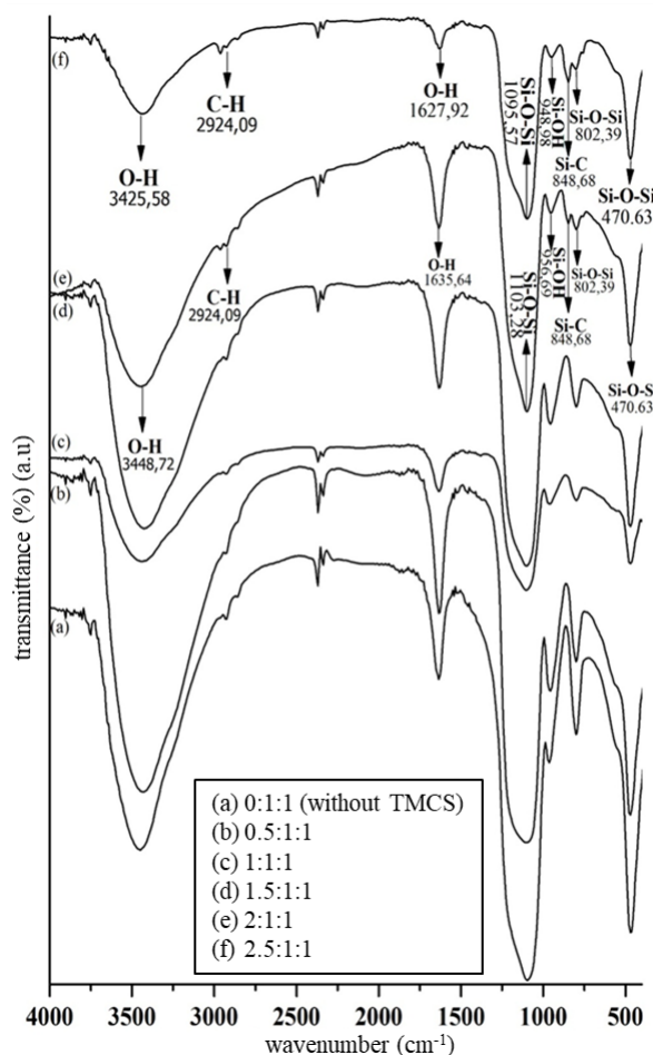
Figure 3. The FTIR spectra of TMCS-modified silica xerogels at volume ratio of TMCS: methanol: PB (a) control; (b) 0.5:1:1; (c) 1:1:1; (d) 1.5:1:1; (e) 2:1:1; (f) 2.5:1:1
