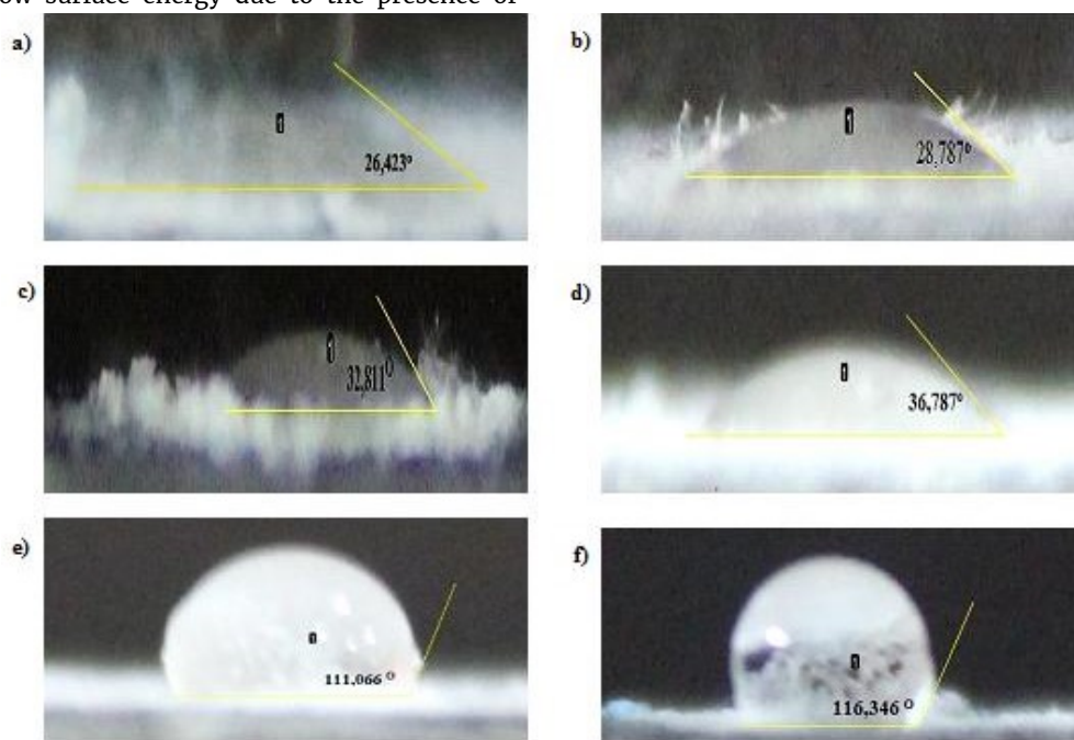
Figure 6. Water contact angles of synthesized silica xerogel at TMCS: methanol: petroleum benzene volume ratio of a) 0:1:1, b) 0.5:1:1, c) 1:1:1, d) 1.5:1:1, e) 2:1:1 and f) 2.5:1:1
