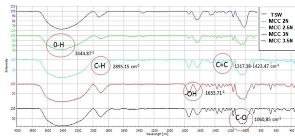
Figure 3. The functional groups of TSW and MCC in the FTIR spectrum.
