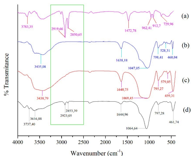
Figure 1. FTIR spectra of (a) HDTMABr, (b) natural zeolite, (c) activated zeolite after milling process, and (d) HDTMA-modified natural zeolite.
