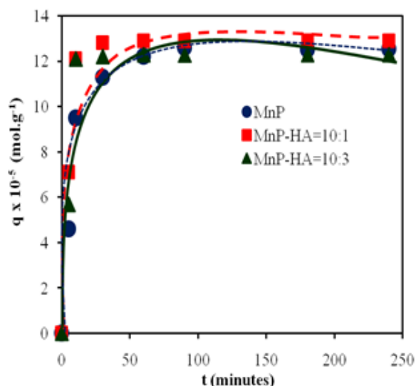
Figure 7. Effect of contact time on the removal of [\text{AuCl}_4]^- using MnP, MnP-HA=10:1 and MnP-HA=10:3
