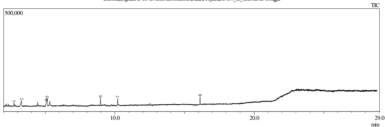
Chromatogram C 80 C:\GCMSsolution\Data\Project2\1437_C_GCMSVC 80.qgd
