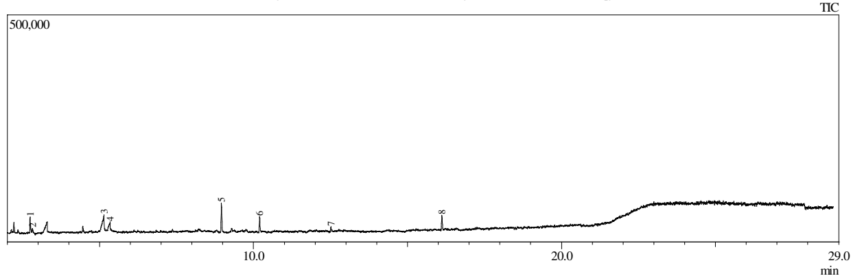
Chromatogram C 90 C:\GCMSsolution\Data\Project2\1437_C_GCMSVC 90.qgd
