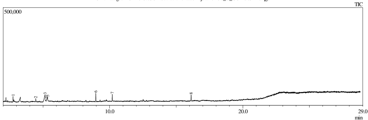
Chromatogram C 140 C:\GCMSsolution\Data\Project2\1437_C_GCMSVC 140.qgd
