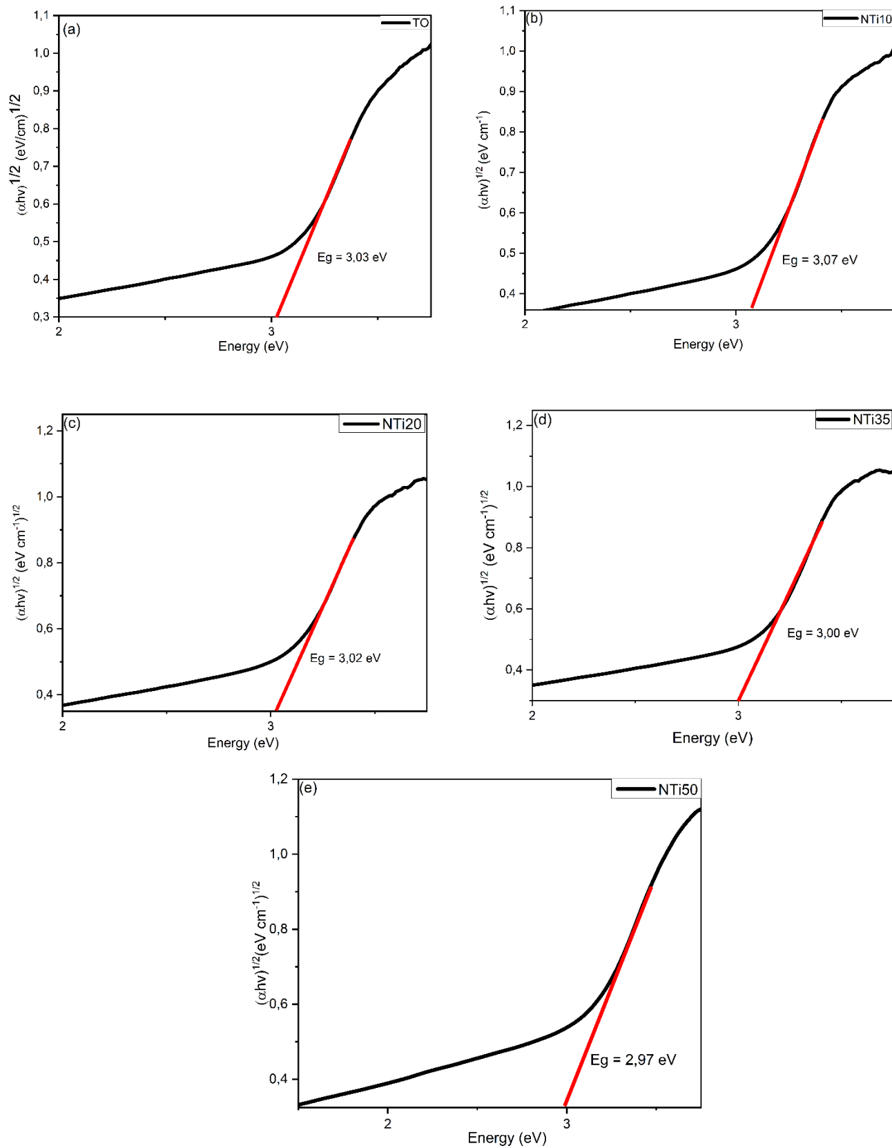
Figure S1. The Bandgap energy ( E_g ) of: a) TO, b) NTi10, c) NTi20, d) NTi35, e) NTi50
