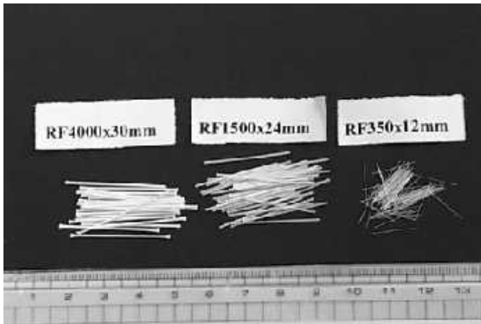
Figure 1. PVA Fibers manufactured for FRC
