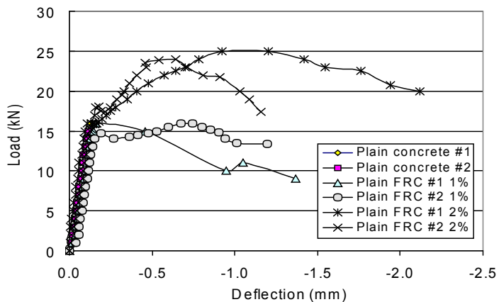
Figure 2. Load-Deflection Relationship of Beam Specimen
