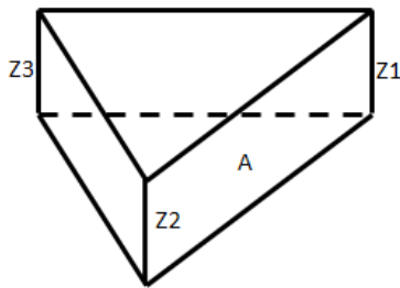
Gambar 3. Perhitungan volume DTM
