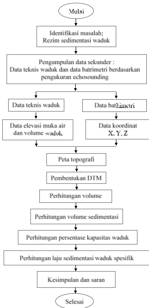
Gambar 4. Alur Penelitian
