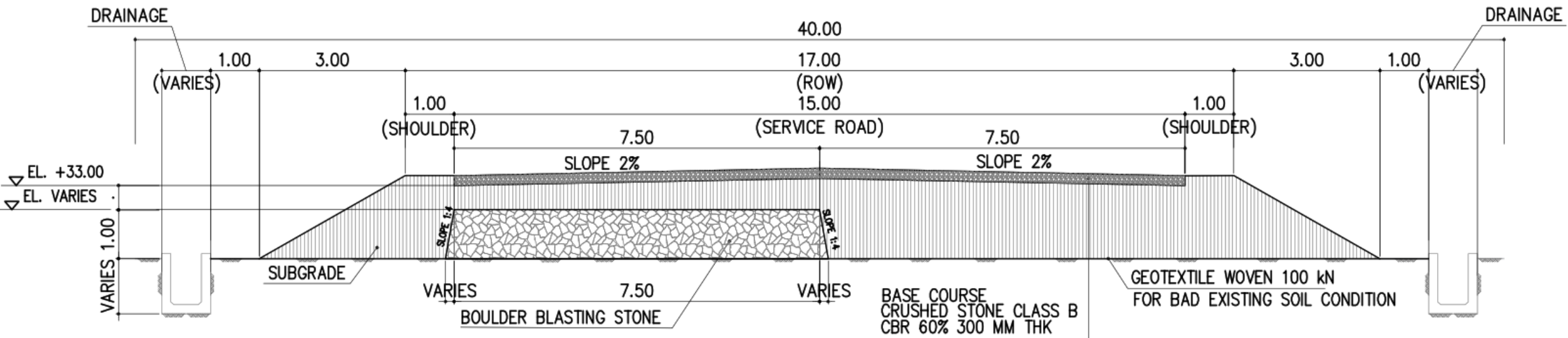
Modification Road Subgrade Method with material replace (2 nd option)
