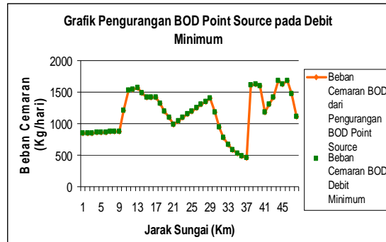
Gambar 13 Hasil Simulasi Pengurangan Cemaran BOD Menu Point Loads And Withdrawal
