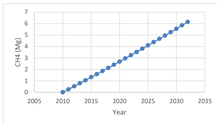
Figure 2. Total methane production in Klotok Landfill in 2010-2032
