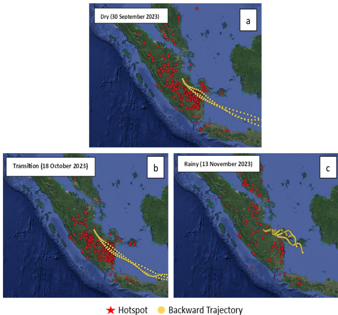
Figure 5. The air mass backward trajectories to Jambi City in each season of PM 2.5 maximum levels (a) dry; (b) transition; (c) rainy
