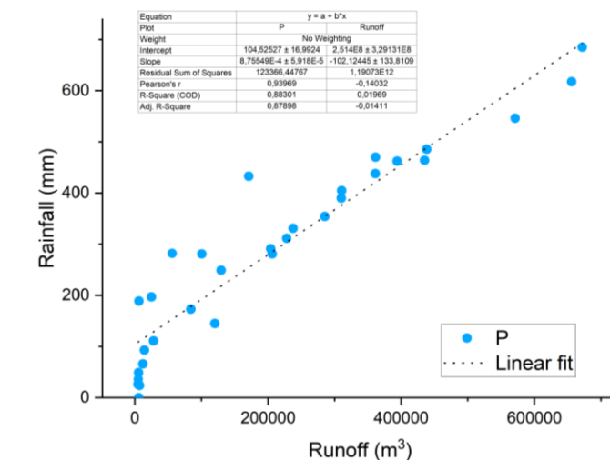
Figure 6. Rainfall–runoff correlation
