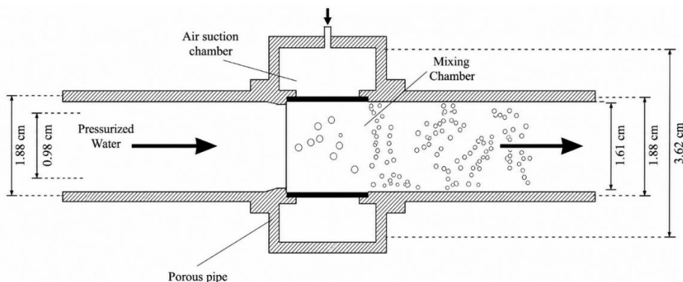
Figure 2. Schematic of the porousVenturi microbubble generator (Majid et al., 2018).
