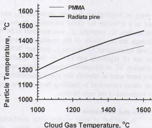
Figure 1. Particle temperatures of Radiata pine and PMMA soots within a binary-species cloud (base-case calculations) as a function of the cloud gas temperature.
