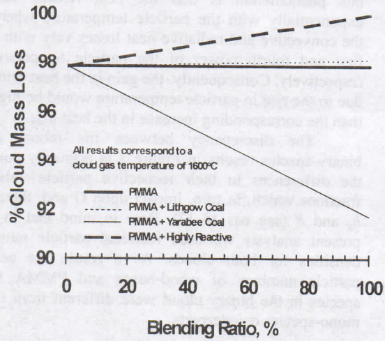
Figure 9. Effect of the mixing ratio on %CML for binary-species clouds of PMMA and several coal soot species.
