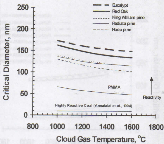
Figure 8. Effect of the fuel type (reactivity) on the critical diameter of soots particles in mono-species soot clouds of various fuels.
