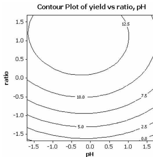
Figure 9. Contour of pH and ratio influence to rendement at temperature 150°C
