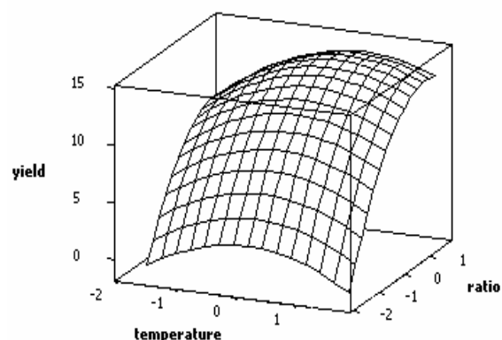
Figure 8. Surface response of temperature and ratio influence to rendement at pH 4.7
