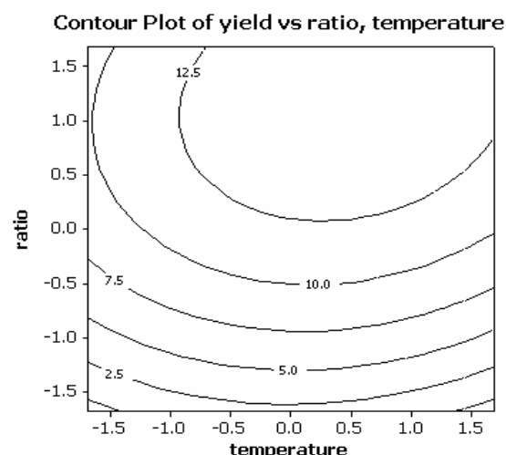
Figure 7. Contour of temperature and ratio influence to rendement at pH 4.7
