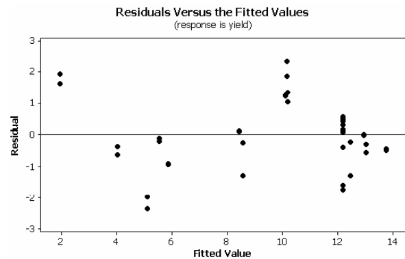
Figure 3. Plot of residual Vs the fitted values
