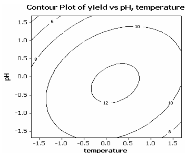
Figure 5. Contour of temperature and pH influence to the rendement at ratio 1:10
