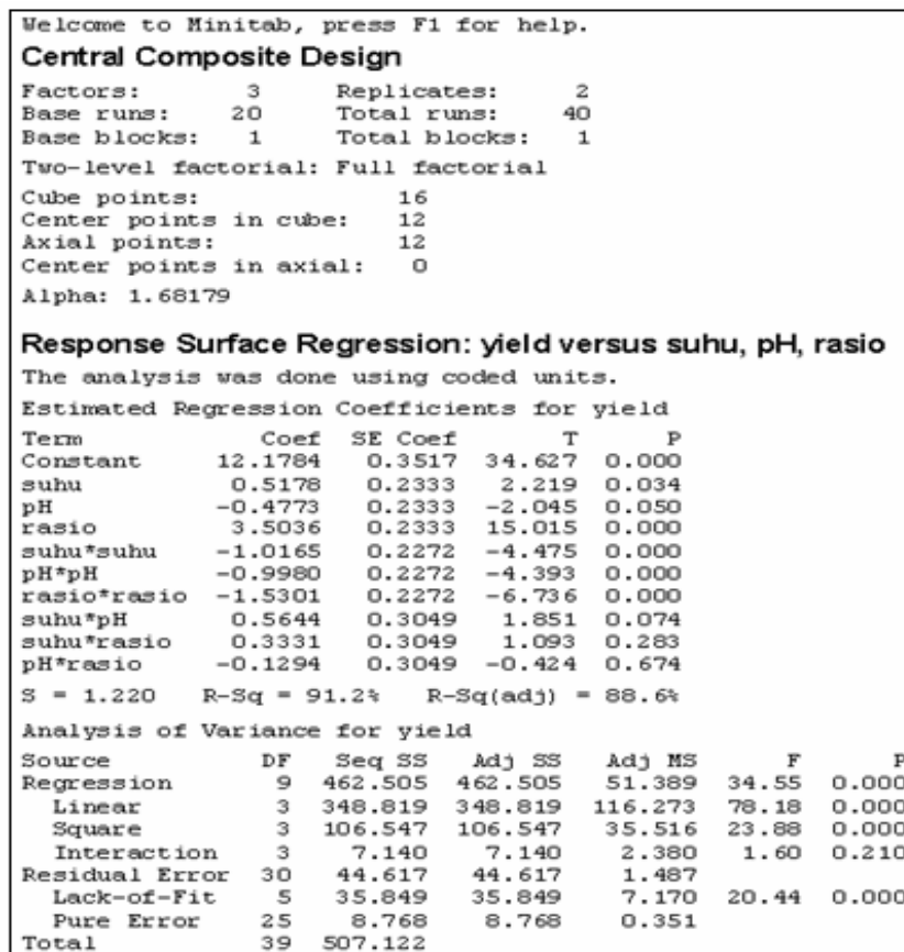
Figure 1. Print out of Minitab 14 analysis result.
