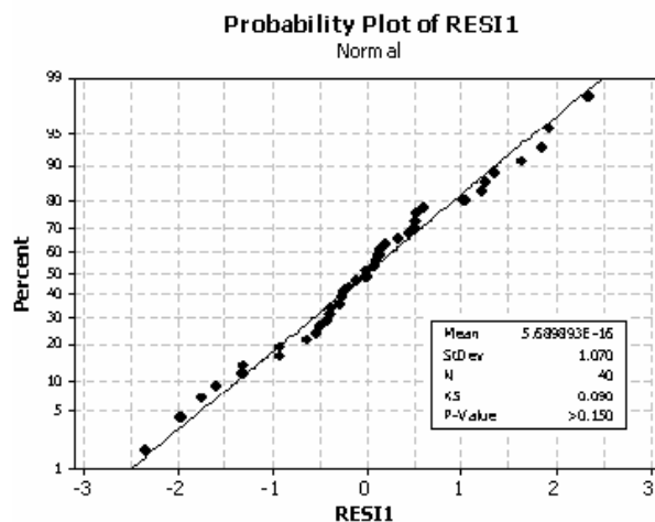
Figure 2. Normality test curve
