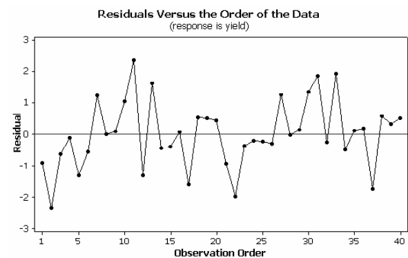
Figure 4. Plot of residual Vs the order of the data
