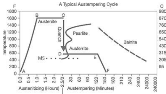
Gambar 1. Proses Austempering
