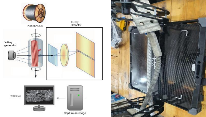
Figure 1. Design of the Reconducting Scheme on ACSR Cables Using X-Ray
