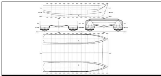
Gambar 2. Lines plan kapal
