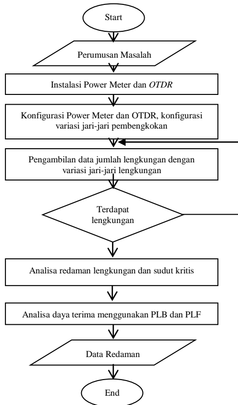
Gambar 3. Flowchart Penelitian
