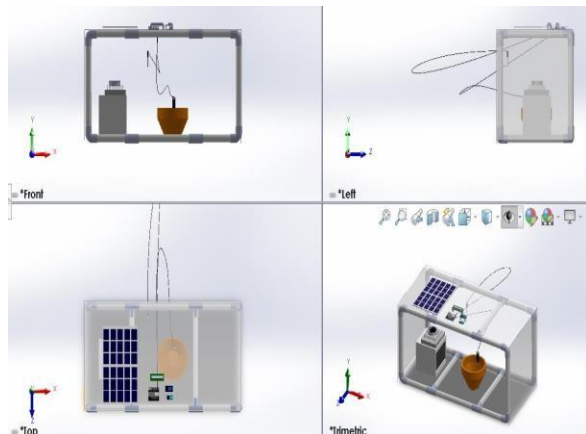
Gambar 10. Desain Prototype Smart Garden
