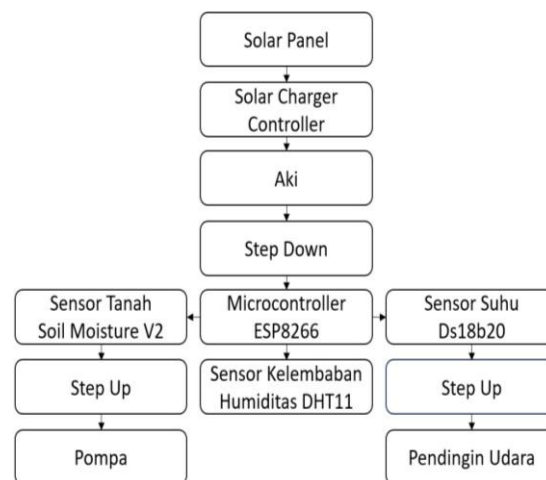
Gambar 8. Flow Chart Sistem
