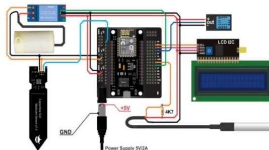
Gambar 9. Skema Sensor Smart Garden
